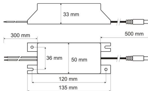
Fig.1. Dimensions of power supply.
